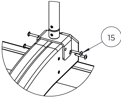
STEP7 SCALE 1:7
