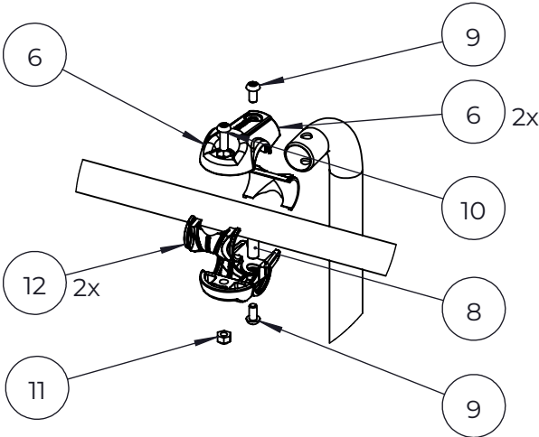
STEP7 SCALE 1:7
