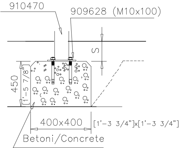
DET 1 OPTION 1 CONCRETE CUBE
