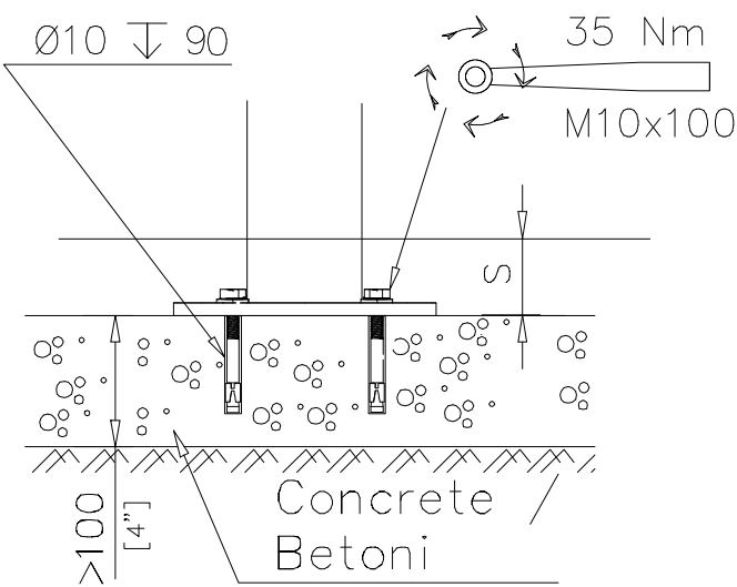
DET 2 OPTION 2 CONCRETE SLAB
