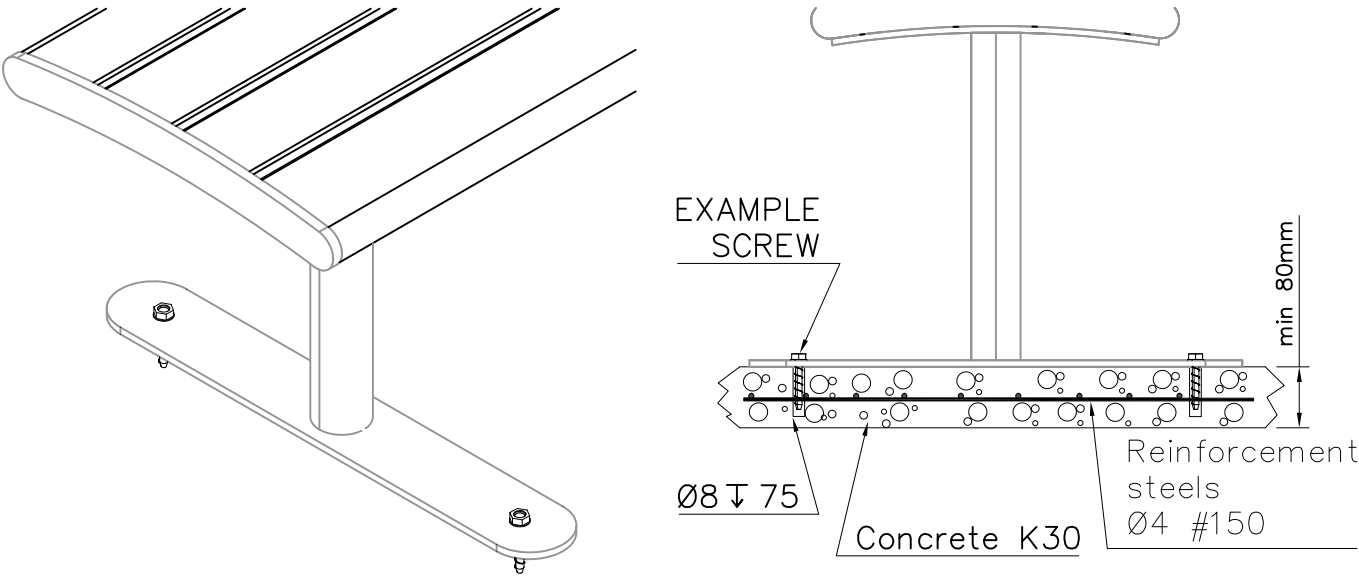
Surface foundation on the ground (BENCHES)
