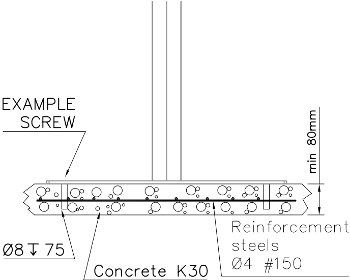
Surface foundation on the ground (CHAIR AND TABLE)
