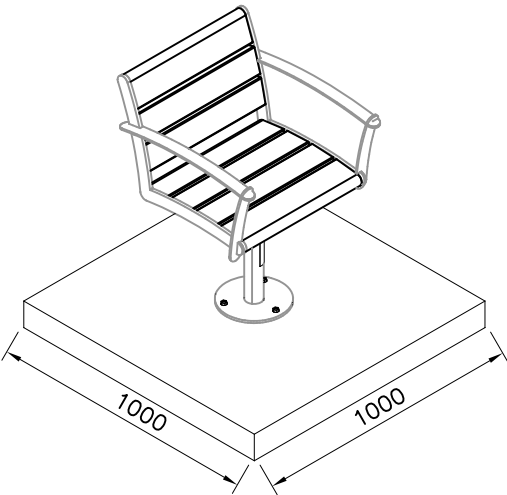
Surface foundation on the concrete plate (CHAIR AND TABLE)
