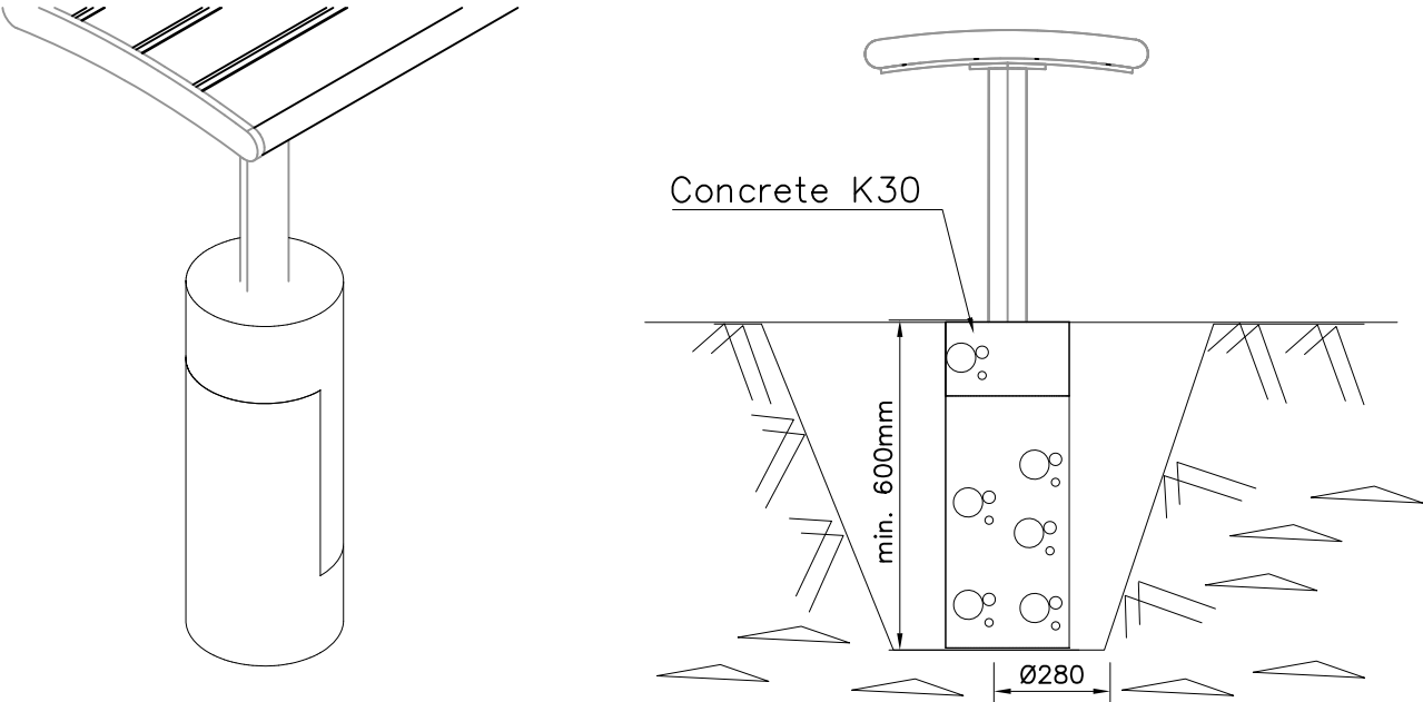
Deep foundation on the ground (BENCHES)
