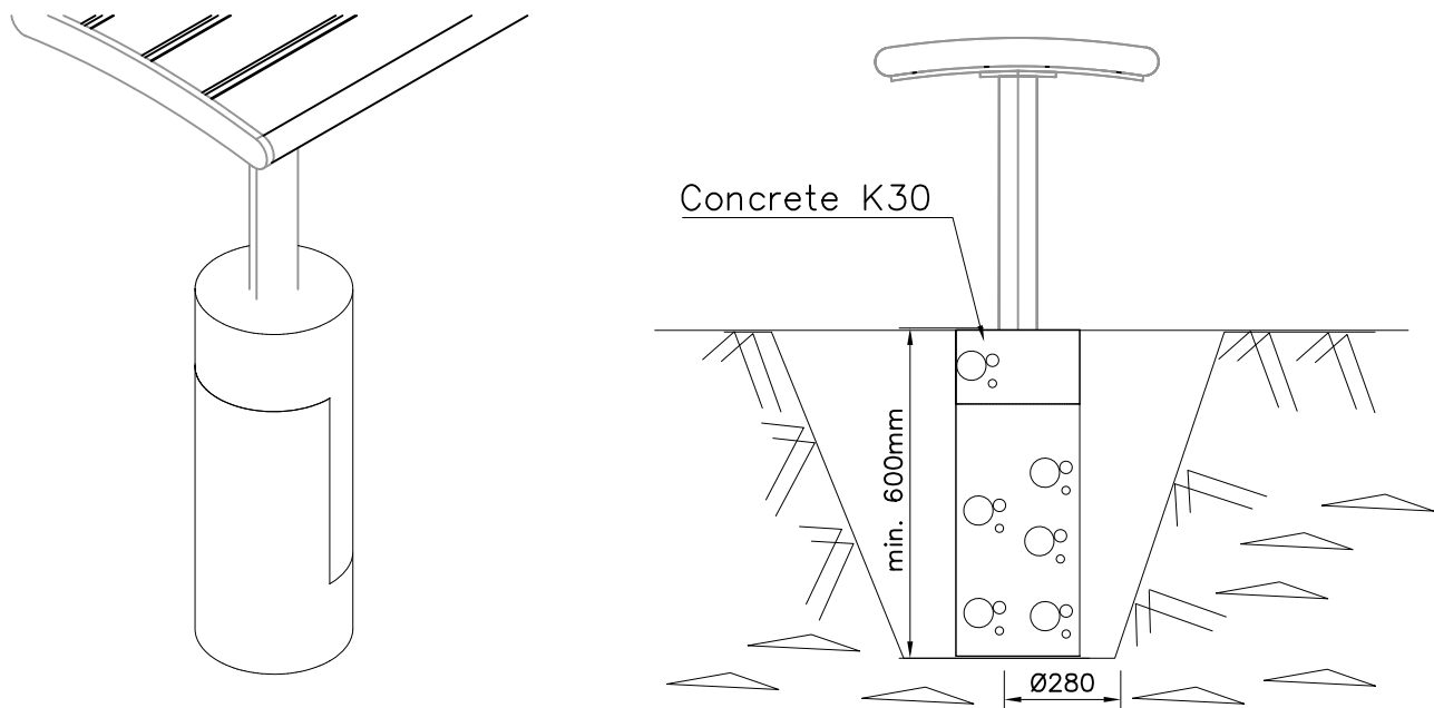
Deep foundation on the ground (BENCHES)
