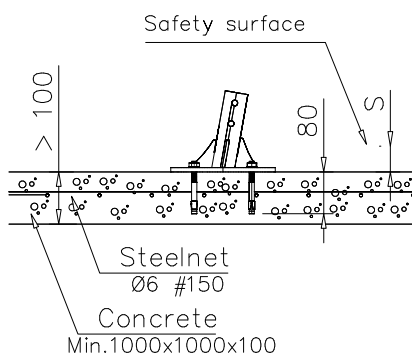
DET 4 DEEP/SURFACE
