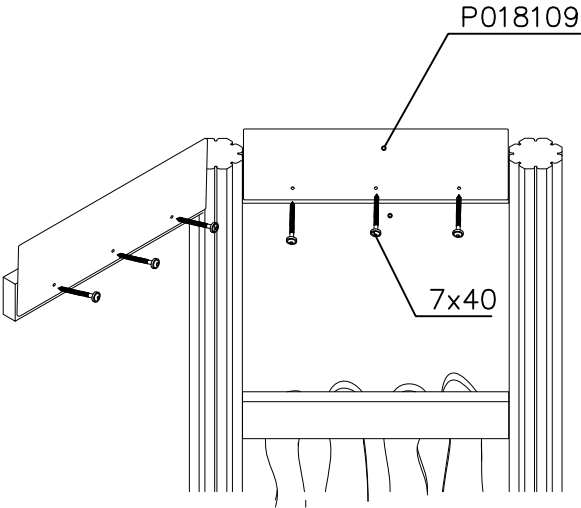
DET 6 – BALCON
