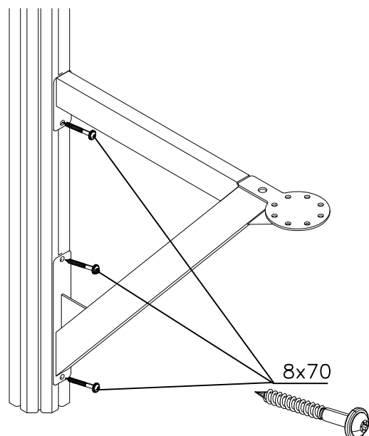
DET 1 – BALCON
