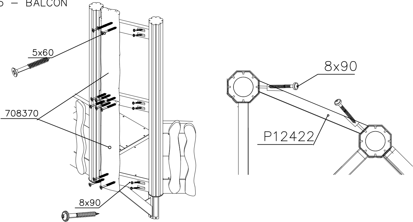
DET 5 – BALCON
