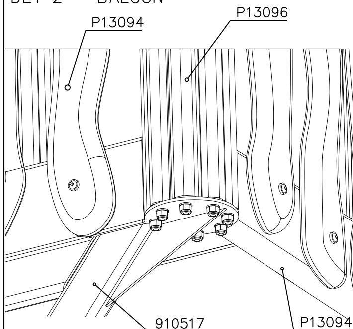
DET 2 – BALCON
